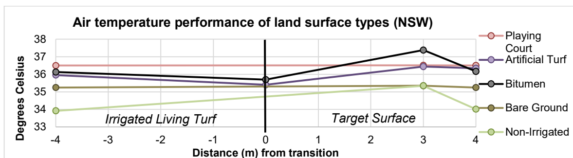
Figure 21. Air temperature results of NSW thermal assessment.
