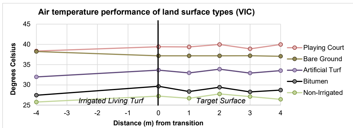
Figure 37. Air temperature results of VIC thermal assessment.
