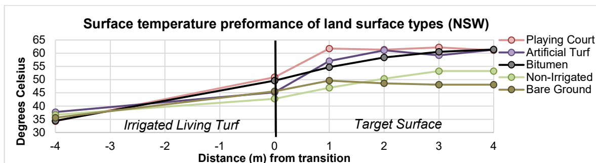
Figure 20. Surface temperature results of NSW thermal assessment.
