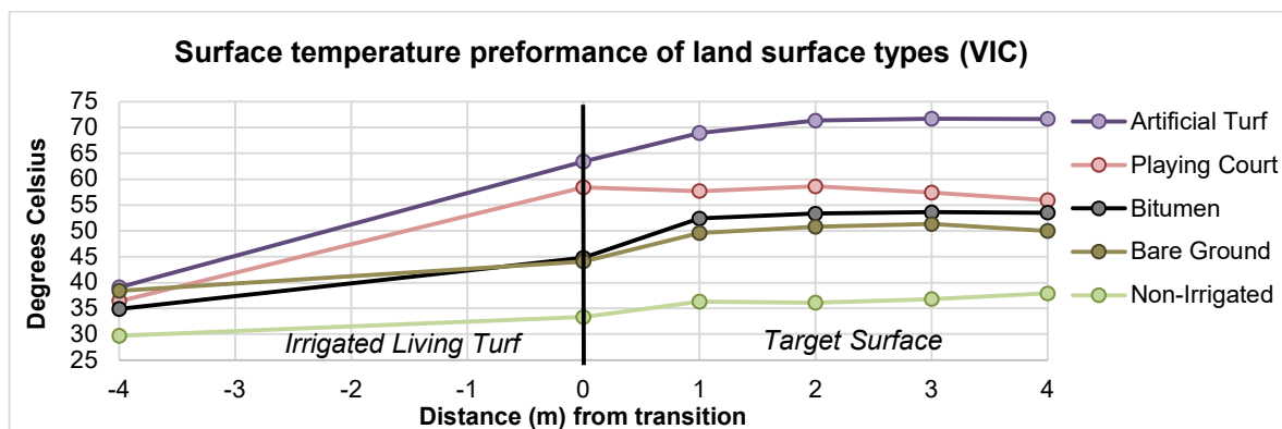
Figure 36. Surface temperature results of VIC thermal assessment.
