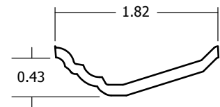
Princeton Smooth Smooth | 6'8" Modified Cove & Bead Sticking
