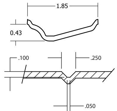
Plank and Groove Detail
