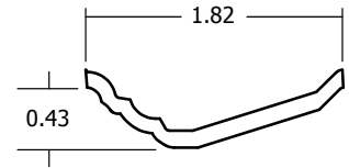
Princeton Smooth Smooth | 7'0" Modified Cove & Bead Sticking
