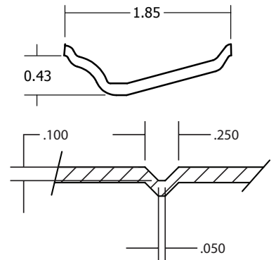
Plank and Groove Detail
