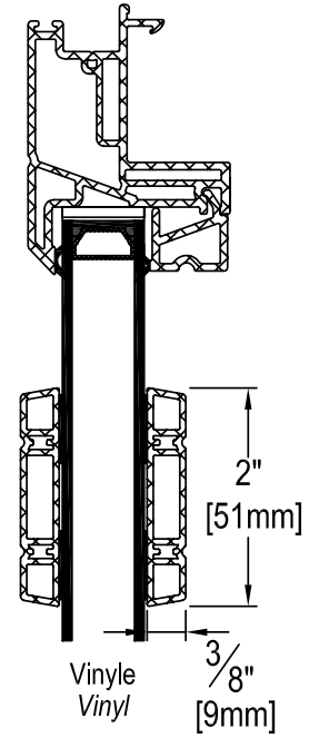
Faux-meneau False mullion
