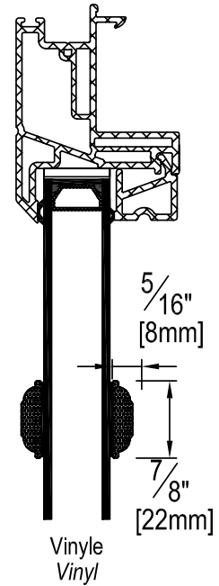
Simili barrotin Simulated divided lite
