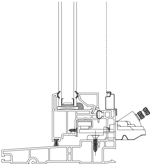
Vertical Section
