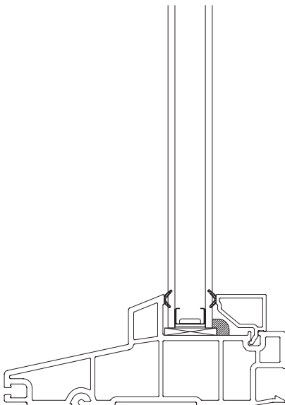
Vertical Section
