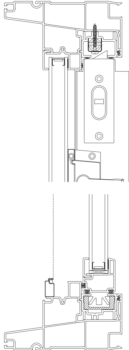
Horizontal Section
