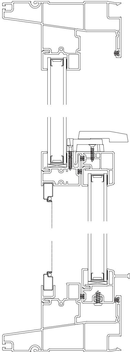
Vertical Section
