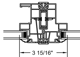
HORIZONTAL MULLION SECTION DETAIL
