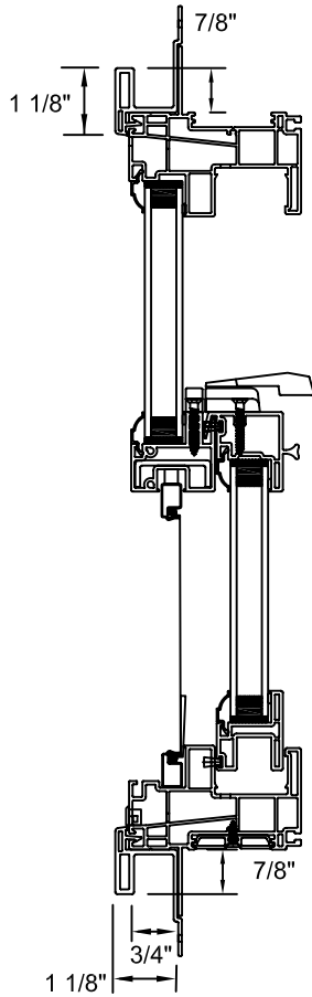
SILL EXPANDER
