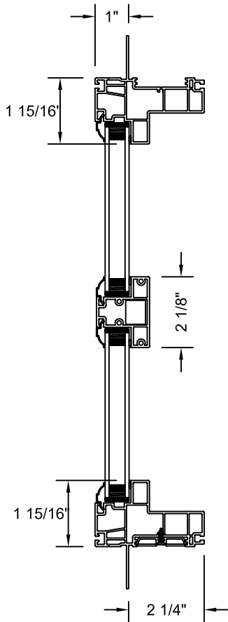
VERTICAL SECTION DETAIL
