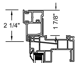
2" BRICKMOULD WITH 1" SILL NOSING
