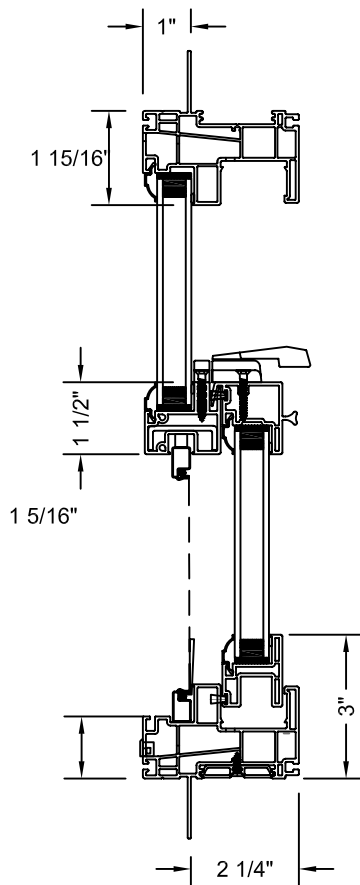
VERTICAL SECTION DETAIL
