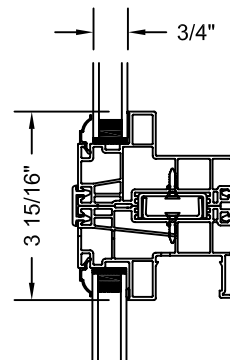
VERTICAL MULLION SECTION DETAIL
