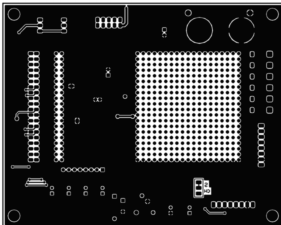
Figure 6. Bottom-side Foil
