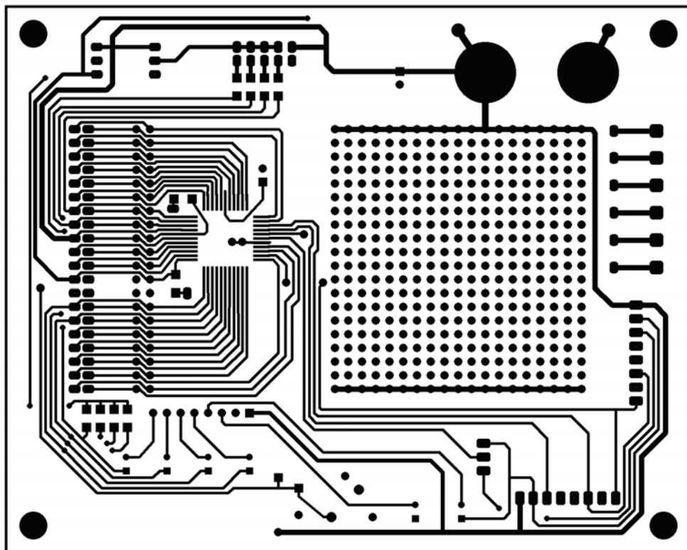
Figure 5. Top-side Foil
