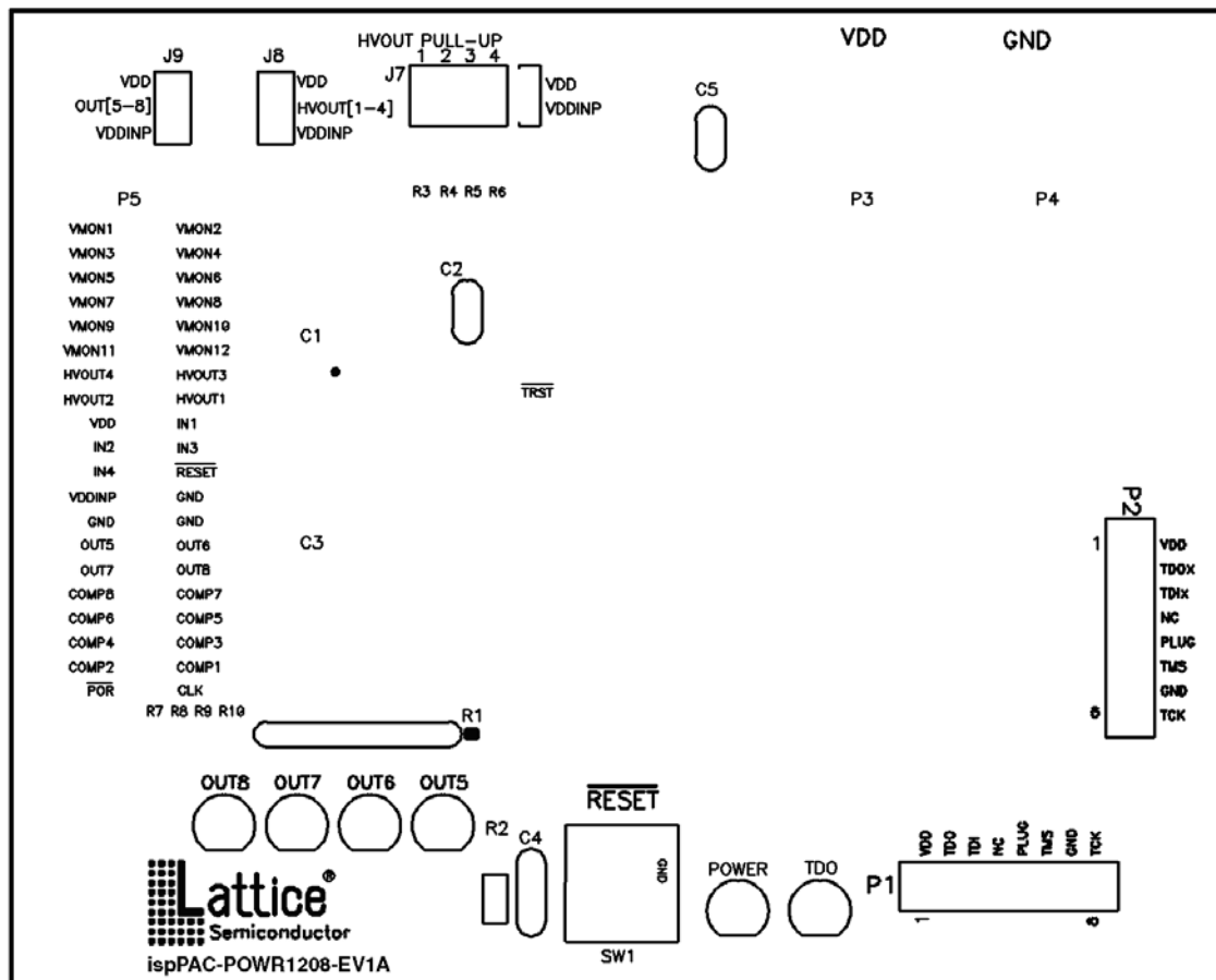
Figure 4. Silk Screen
