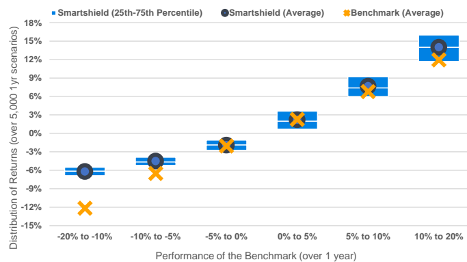
Simulated 1yr performance: Moderate
