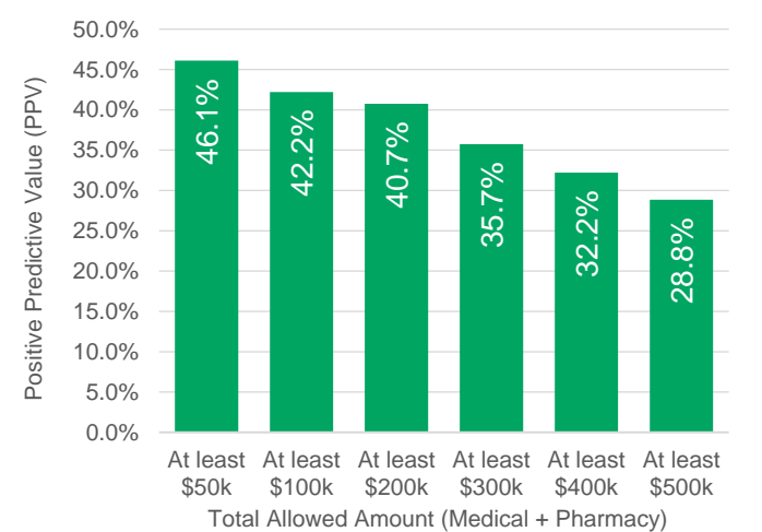
FIGURE 2: PREDICTIVE PERFORMANCE OF PRIOR COST METHOD
