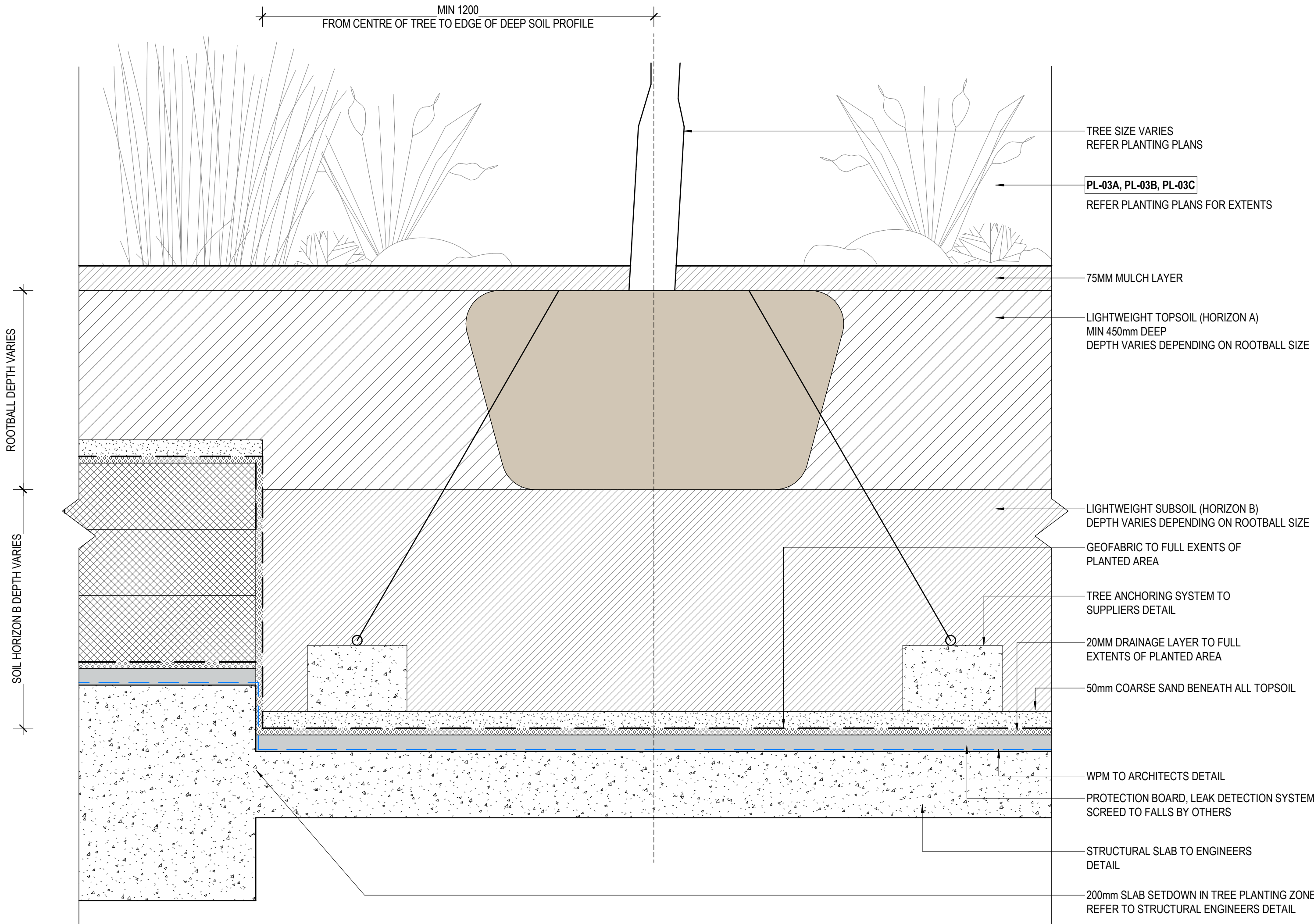
2 TYPICAL SOIL PROFILE - WATERFRONT GARDEN - TREE PLANTING
