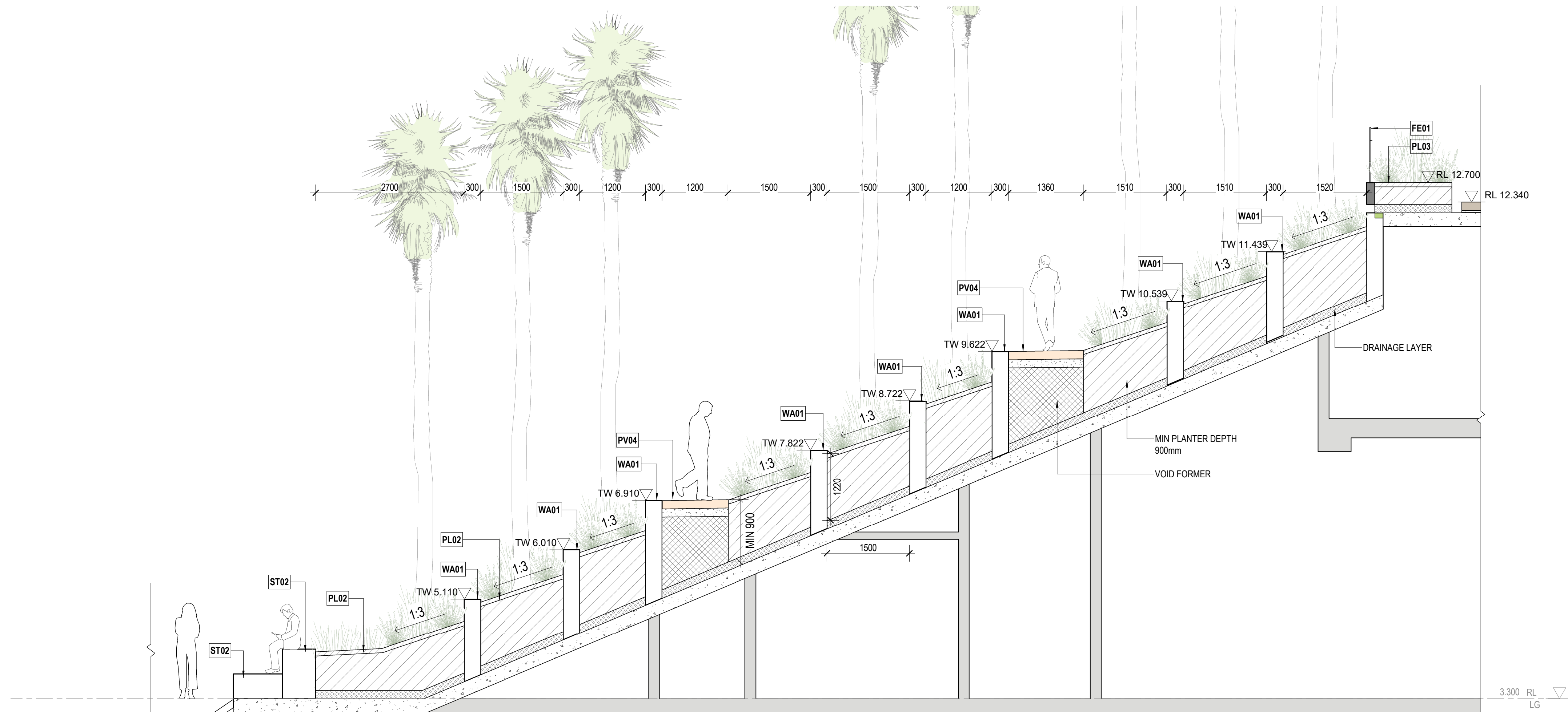
1 WATERFRONT STEPS - SECTION A
