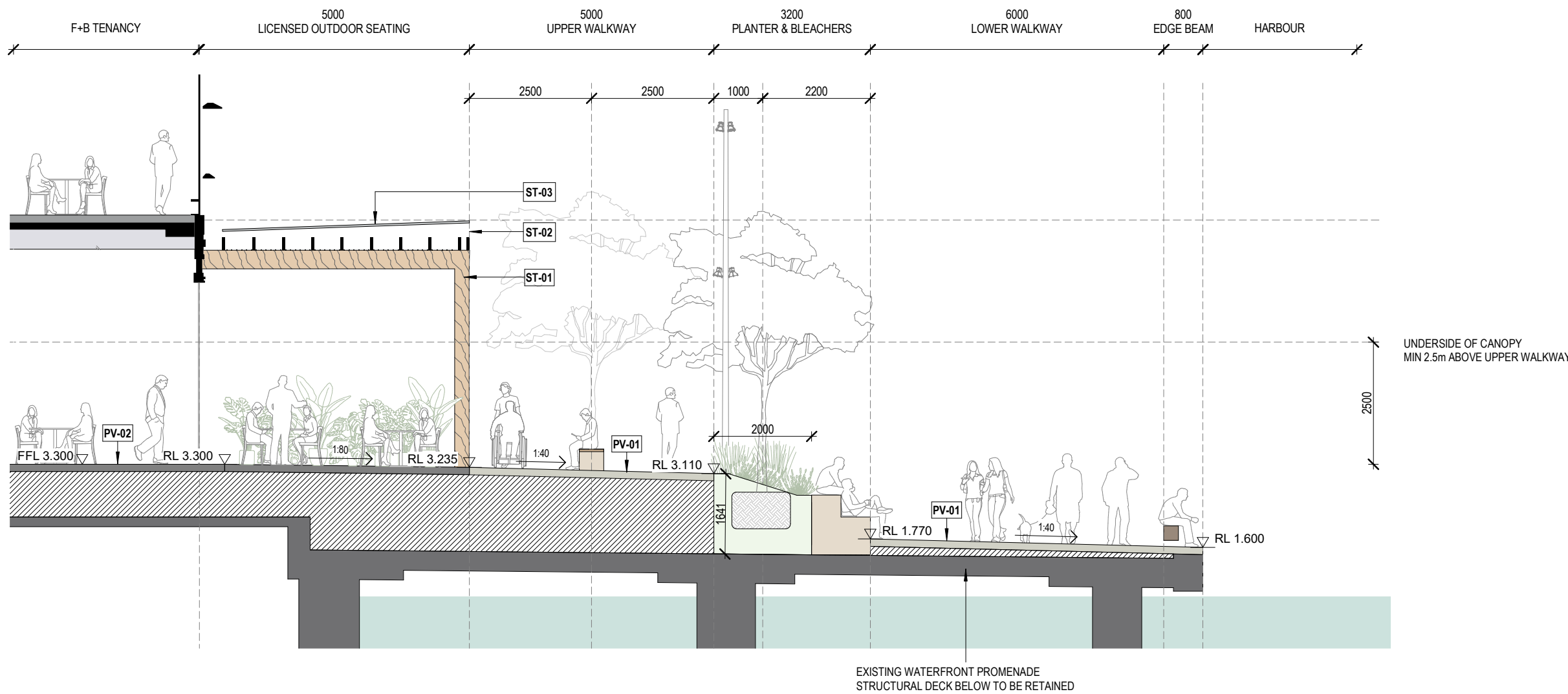
2 Waterfront Promenade - Central Section 1101_05 1:100
