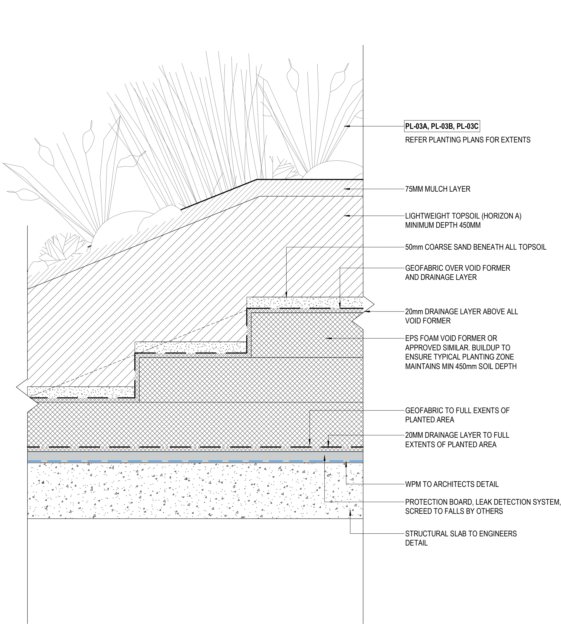
1 TYPICAL SOIL PROFILE - WATERFRONT GARDEN - PLANTING
