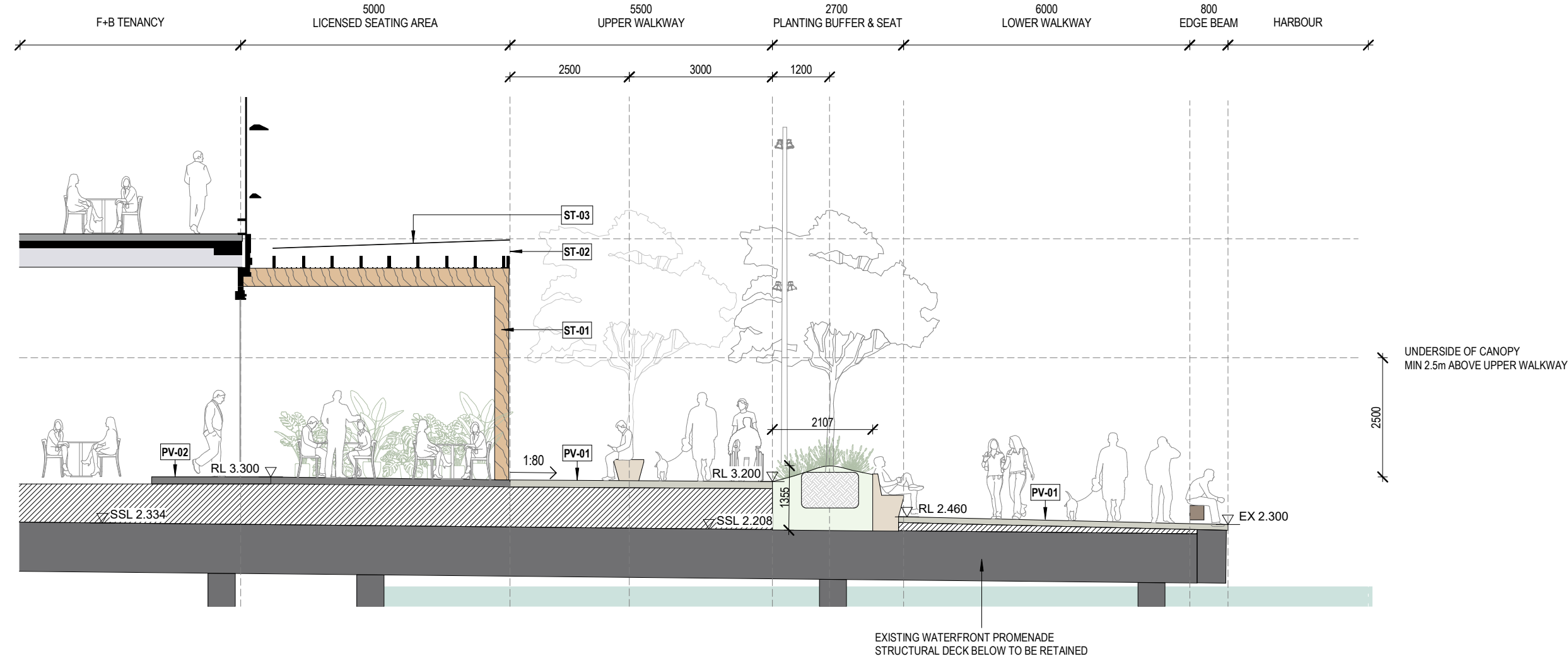
1 Waterfront Promenade - Southern Section 1101_04 1:100
