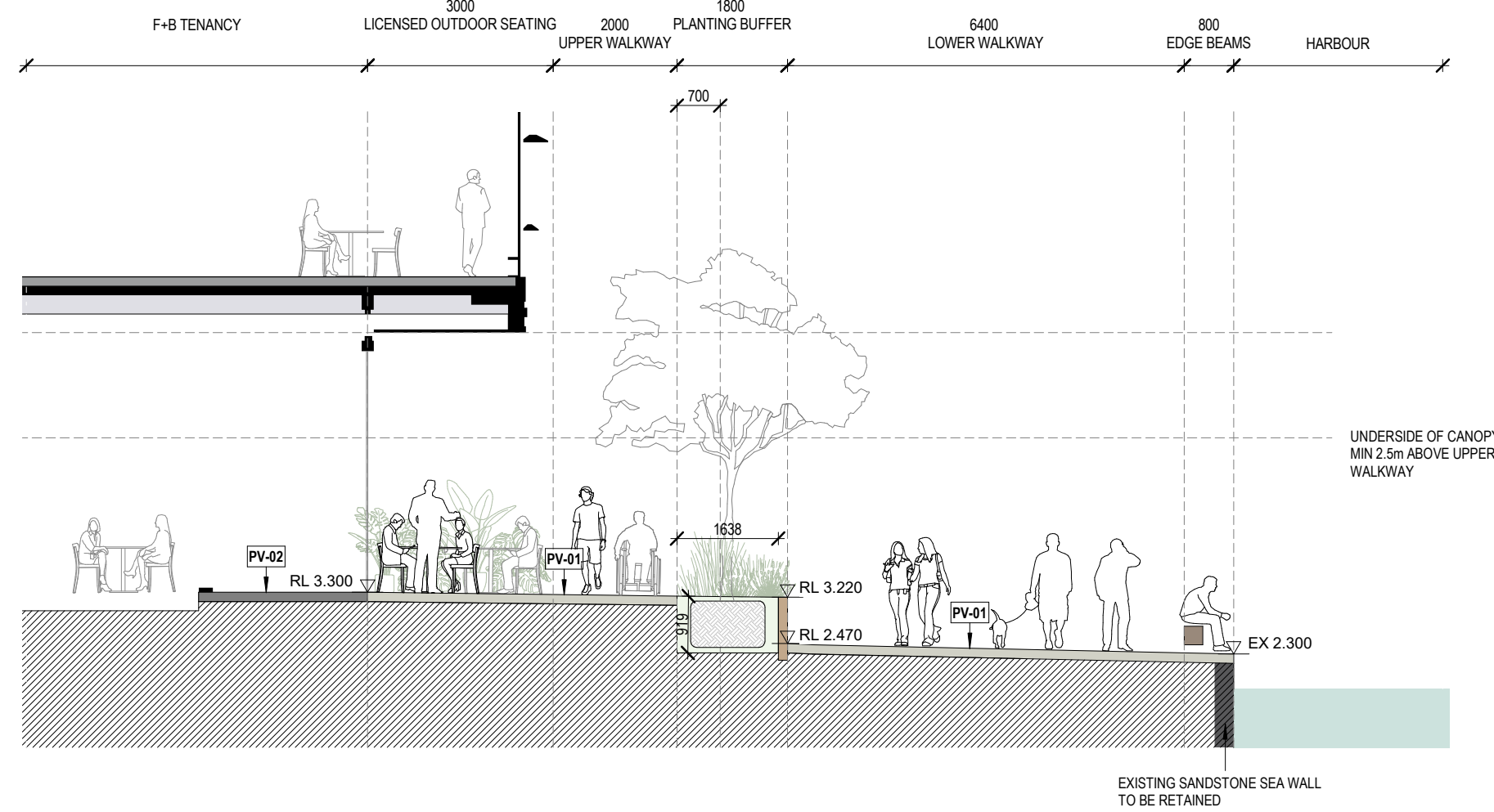
4 Waterfront Promenade - Northern Section 1101_06 1:100
