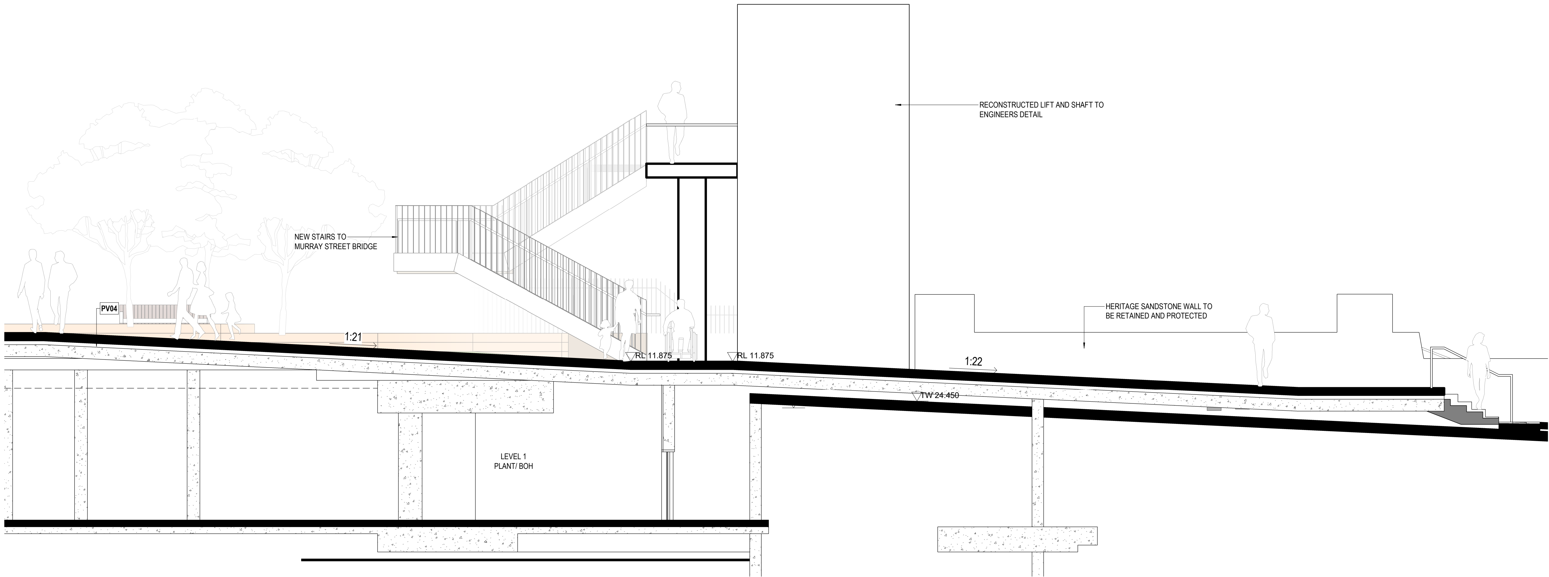
1 WATERFRONT GARDEN NORTH BRIDGE ENTRY SECTION 1102_01 1:50
