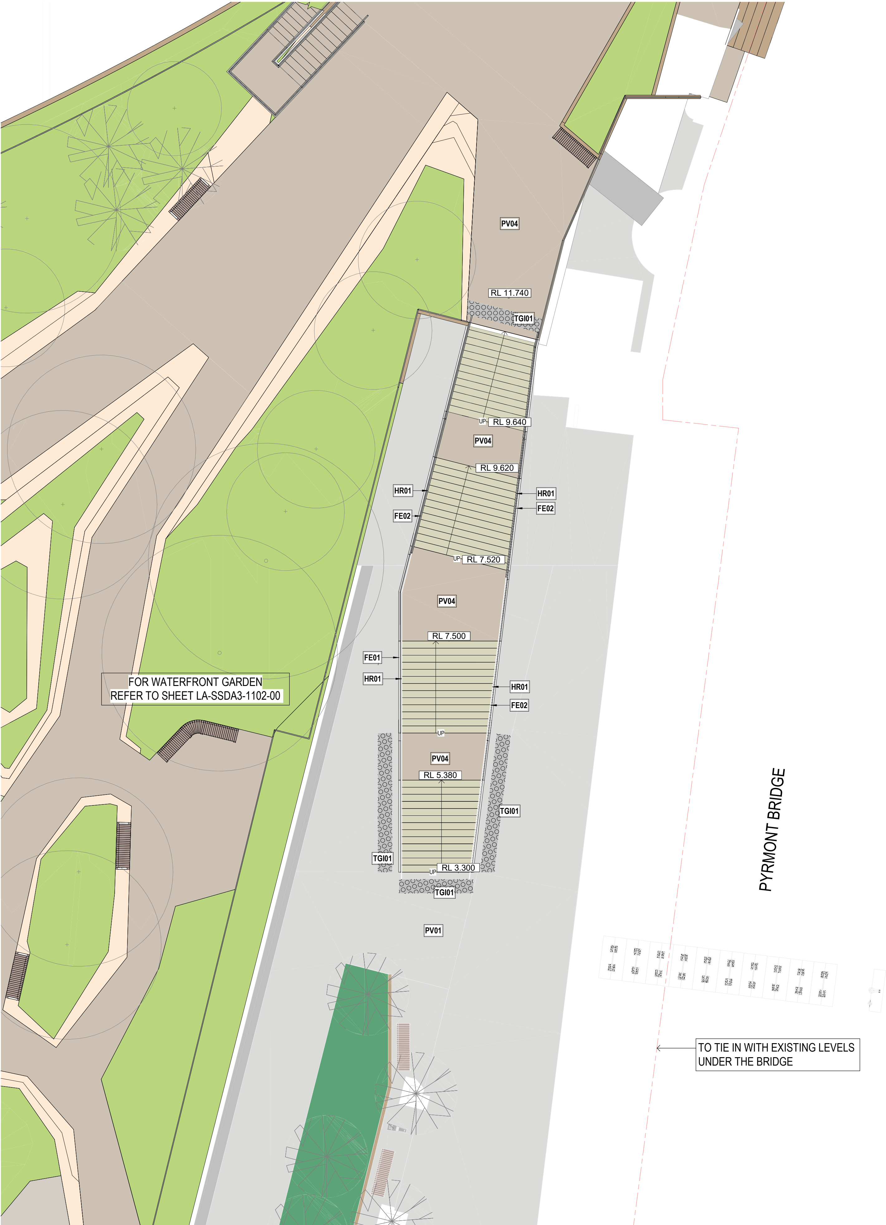
1 PYRMONT BRIDGE STEPS PLAN SK_1102_00 1:100
