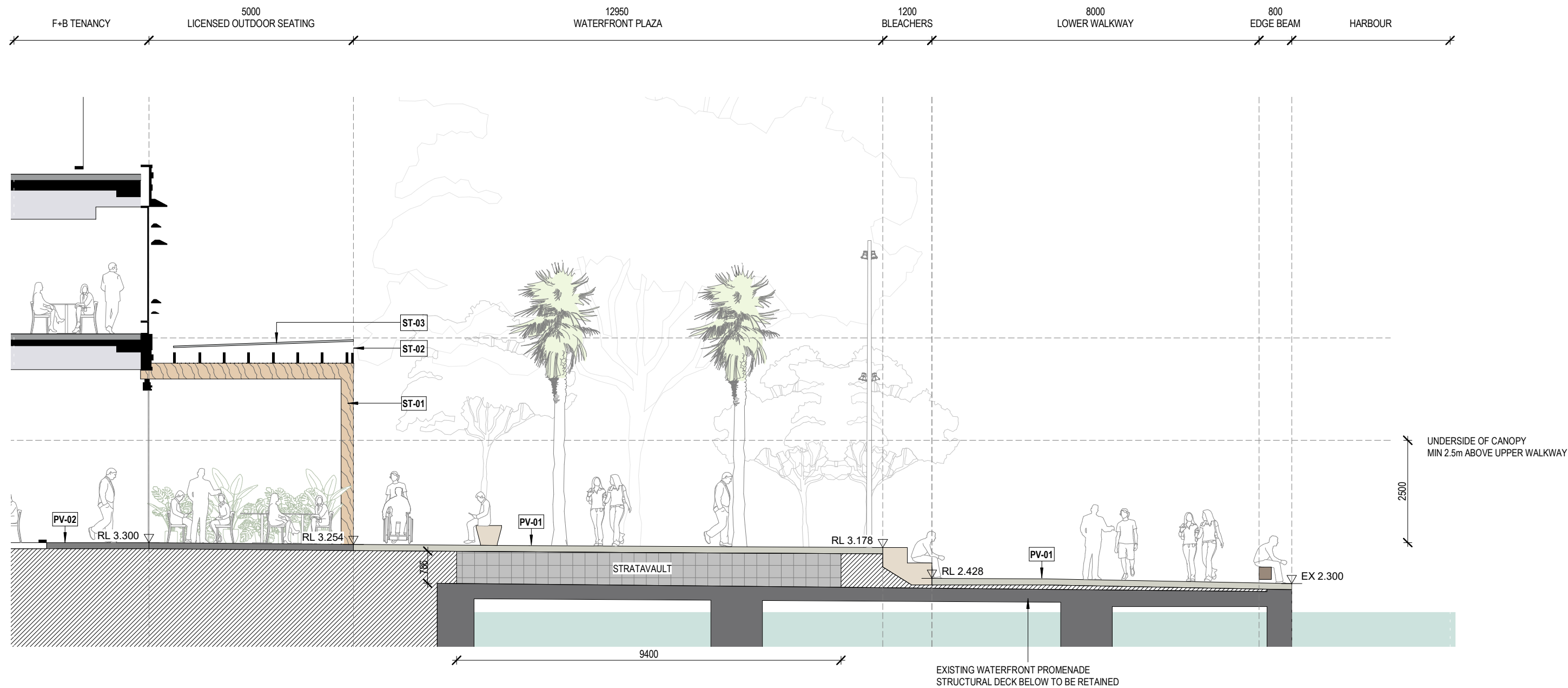
3 Waterfront Promenade - Plaza Section 1101_05 1:100
