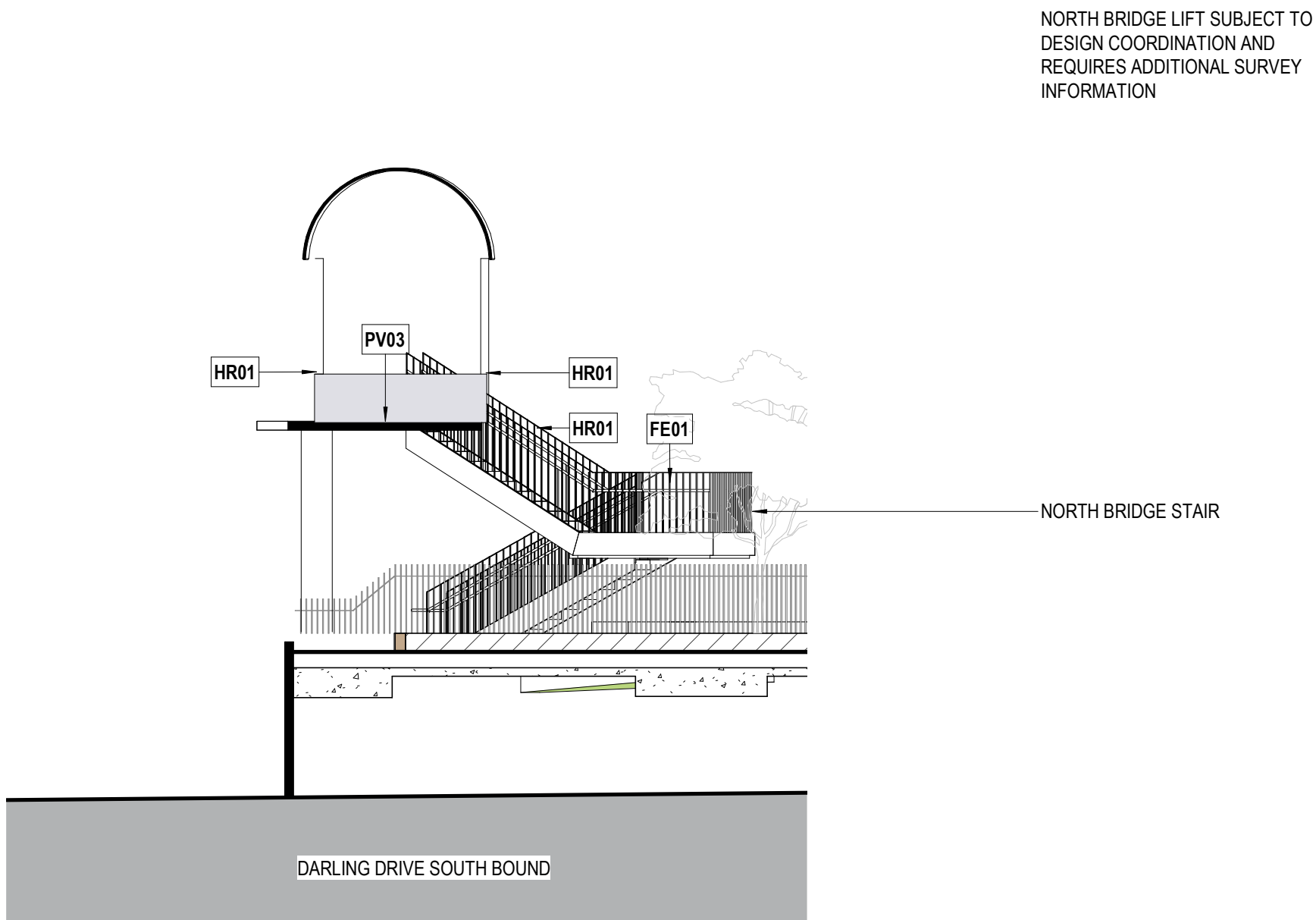
2 NORTH BRIDGE N-S SECTION SK_0015 1:100
