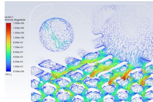
Velocity vector
