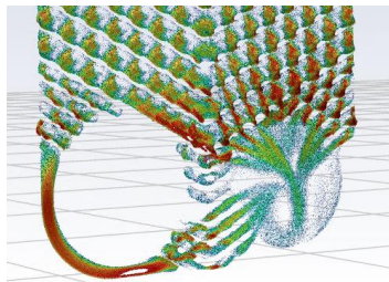
Optimized Flow Distribution Cold Area
