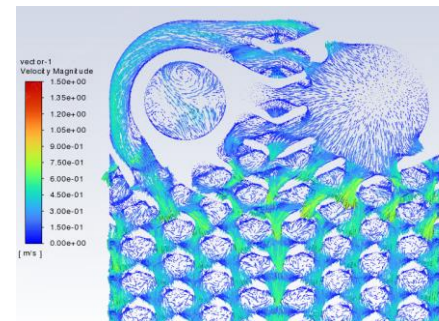
Velocity vector
