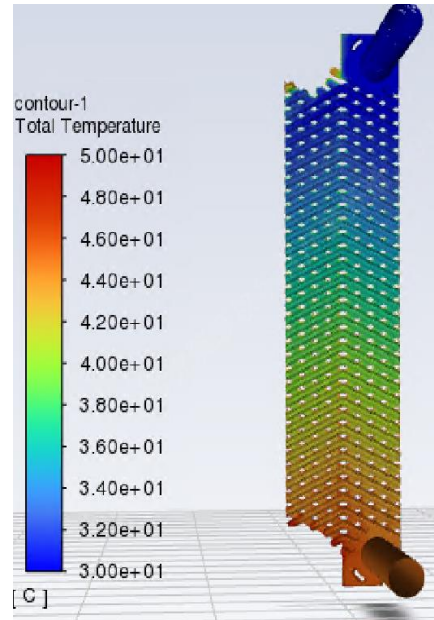
Temperature profile
