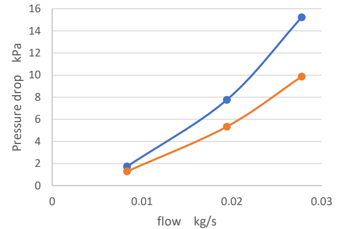
Pressure drop CFD
