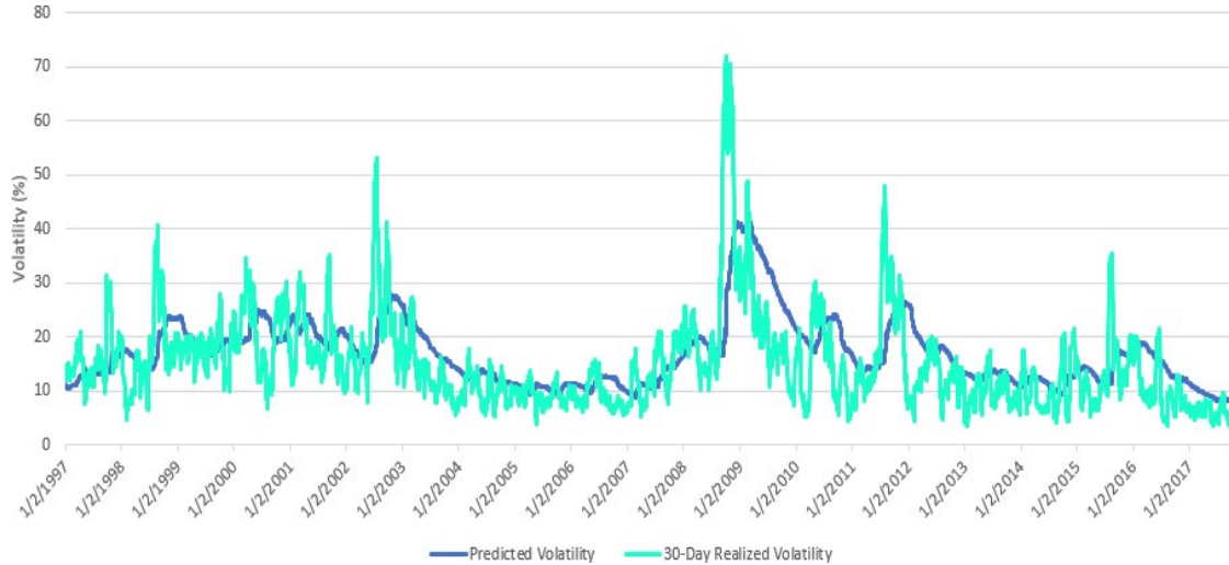
Figure 1: Predicted vs Realized Volatilities: Russell 1000 Index and the Axioma Worldwide Equity Factor Risk Model (AXWW4).
