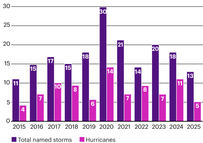
Figure 1. Total named storms and hurricanes, 2015–2025
