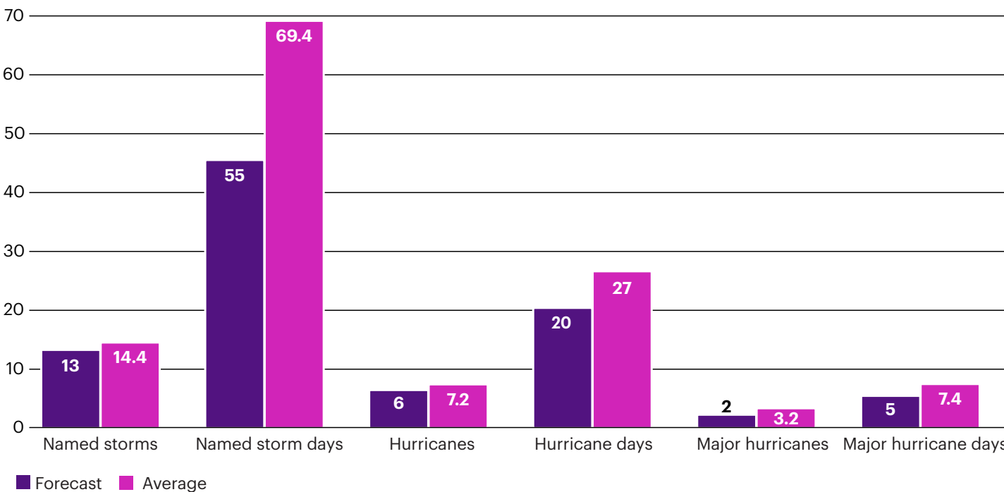
Figure 2. 2026 Hurricane Prediction (Forecast versus Average)
