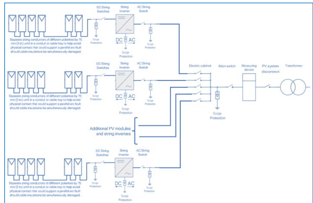
Schematic of a string inverter system (no microinverters and no dc-to-dc converters (optimizers)) with one array connected to each inverter. All inverters are connected to a public utility grid. (Source: ZRS)
