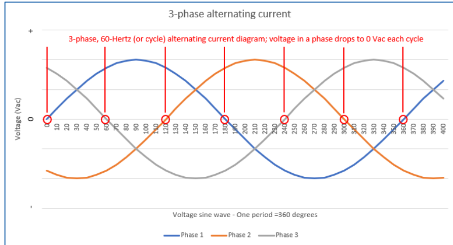
Diagram of alternating current showing a phase at 0 Vac each cycle (this diagram shows a 60 Hz cycle, and 50 Hz would be similar. (Source: ZRS)
